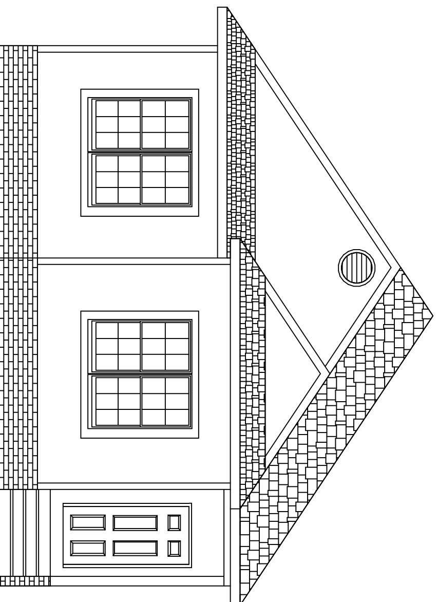
Front Elevation
